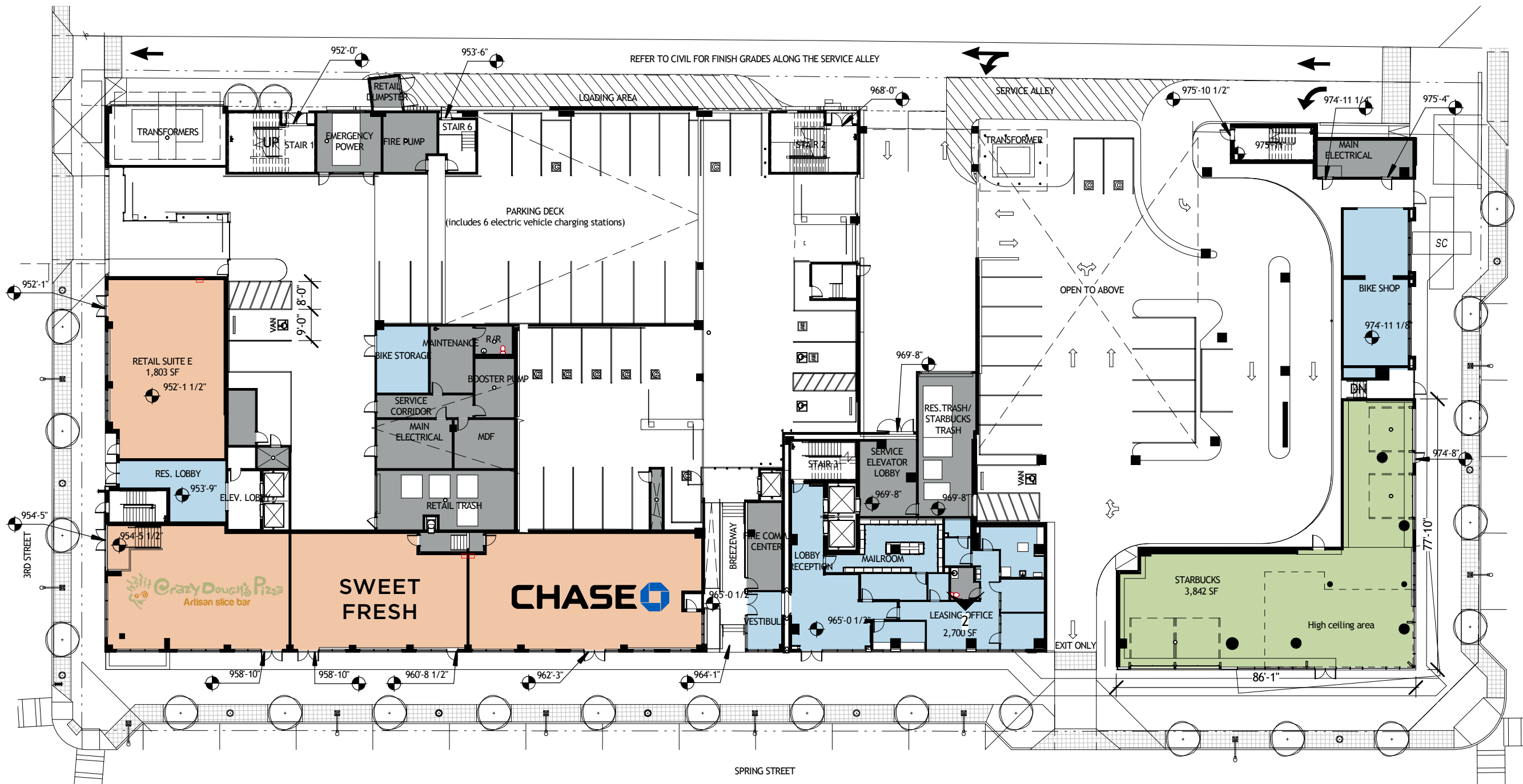
1 RETAIL - SITE PLAN R1.1 1" = 30'-0"
