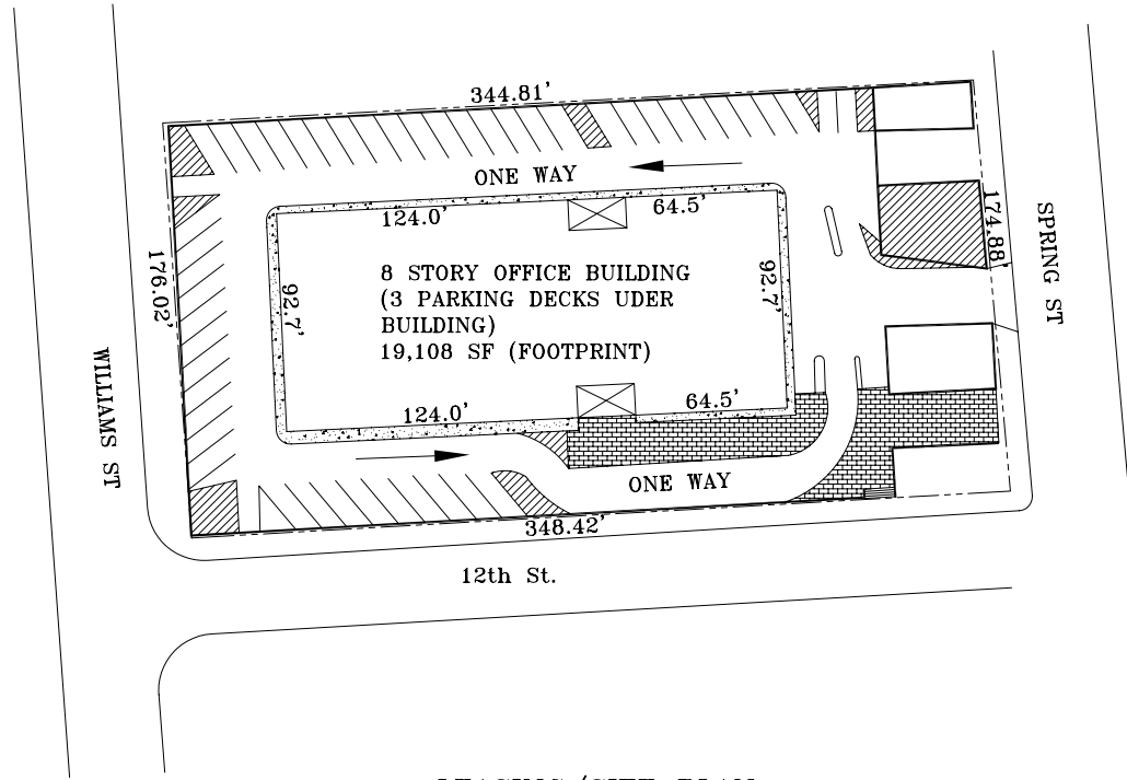
LEASING/SITE PLAN 1"=40'
