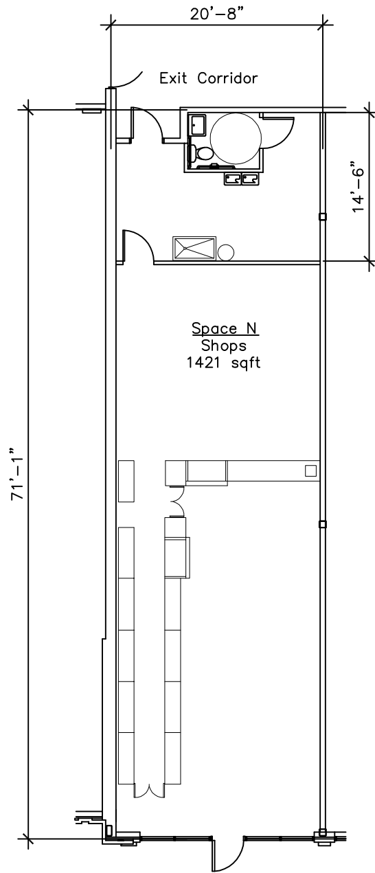
1 FLOOR PLAN SCALE: 1/8"=1'-0"
