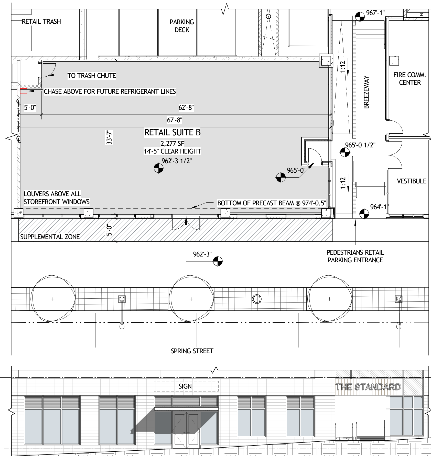
1 RETAIL SUITE B - LOD R1.2 3/32" = 1'-0"
